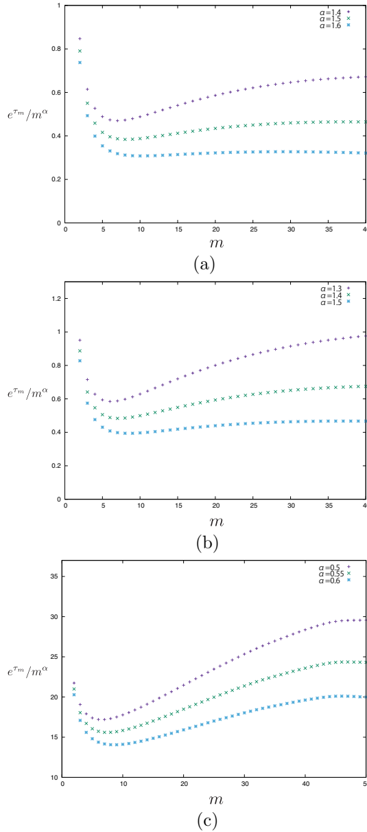
FIG. 3.2. We plot m vs. \exp(\tau_m)/m^\alpha . (a) a = \pi, u_0(x) = 0.5(\cos(x/2) + \sin^2 2x) ( \alpha = 1.4, 1.5, 1.6 ), (b) a = \pi, u_0(x) = 0.5(\cos(x/2) + \sin^2 4x) ( \alpha = 1.3, 1.4, 1.5 ). (c) a = 2\pi, u_0(x) = \sin\left(\pi\left(\frac{x}{2\pi}\right)^8\right) + 0.01 \cos(x/4) ( \alpha = 0.5, 0.55, 0.6 ).
