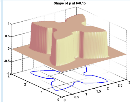
Figure 4.1. Shape of the solution for Example 1.
