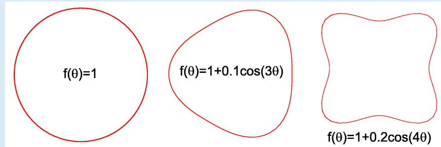
Figure 2.1. The Frank diagram of anisotropy.
