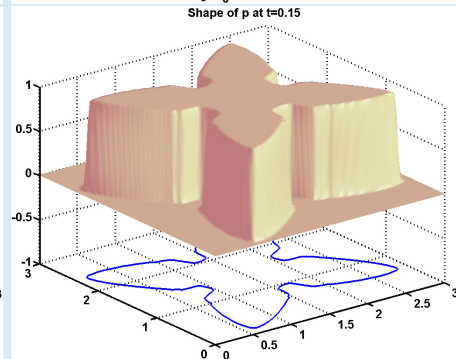
Figure 4.3. Shape of the solution for Example 2.
