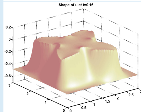
Figure 4.1. Shape of the solution for Example 1.
