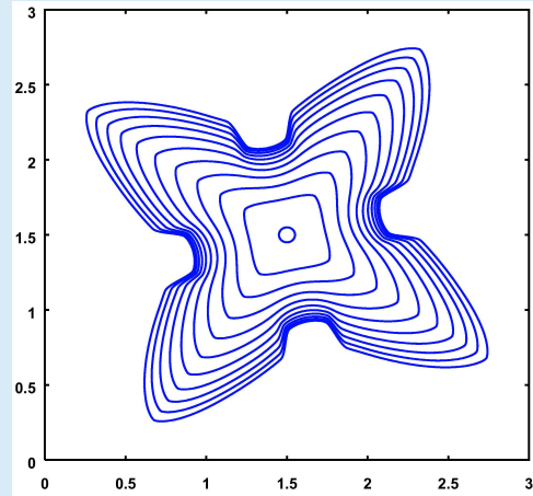
Figure 4.2. Evolution of the level set \frac{1}{2} for Example 1.
