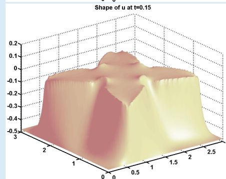
Figure 4.3. Shape of the solution for Example 2.
