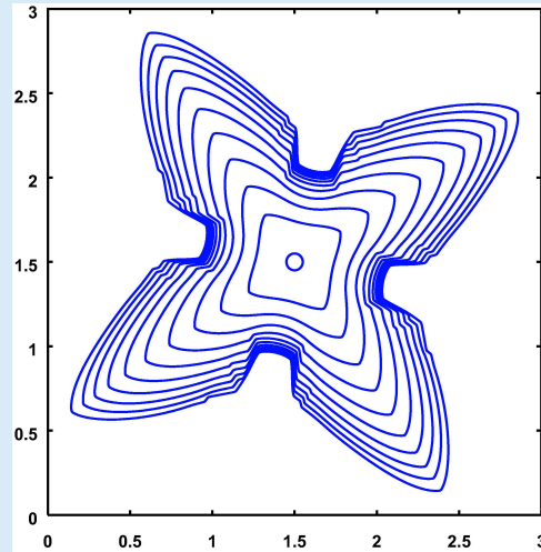
Figure 4.4. Evolution of the level set \frac{1}{2} for Example 2.
